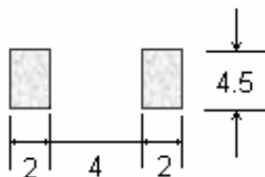
WI-5650 PCB PATTERN
